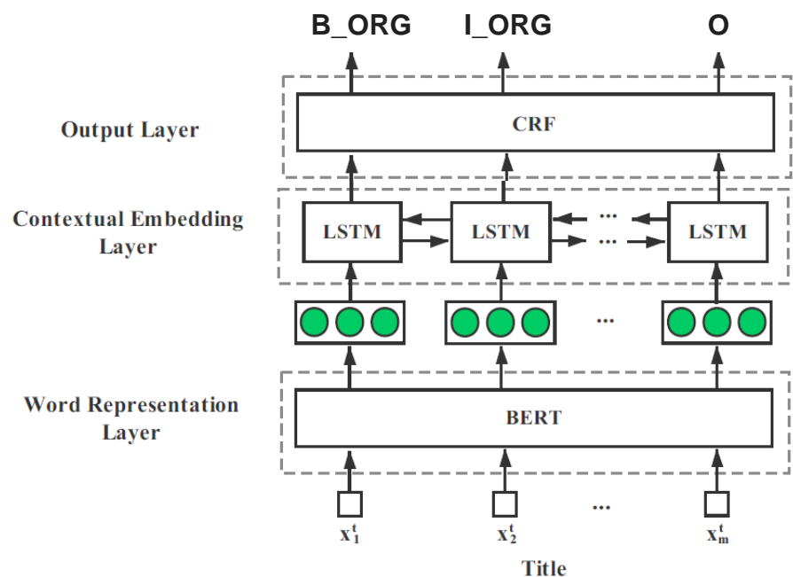
BERT+Bi-LSTM+CRF
